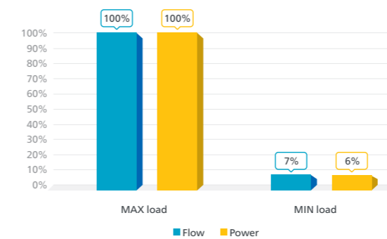
Oil-injected screw with VSD
