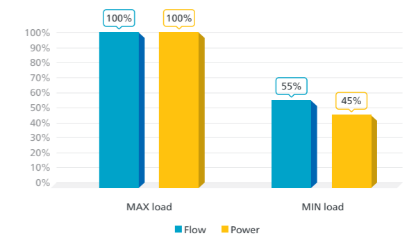
Typical oil-sealed rotary vanes with VSD
