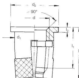
Type 0231 Ⓢ EXPANSIONsert 1 flange
