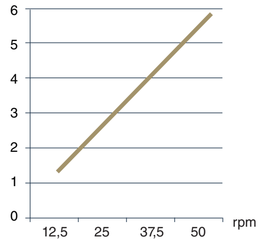
Q [l/min.] LSM-15
